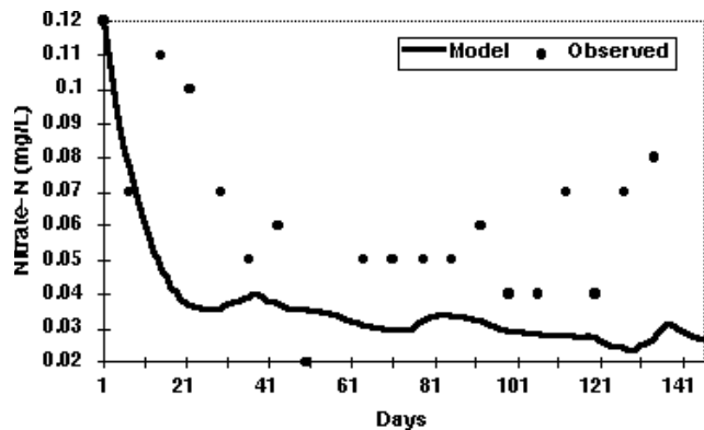
Figure 5. Water column nitrate nitrogen simulation for the Butare site in Rwanda.
