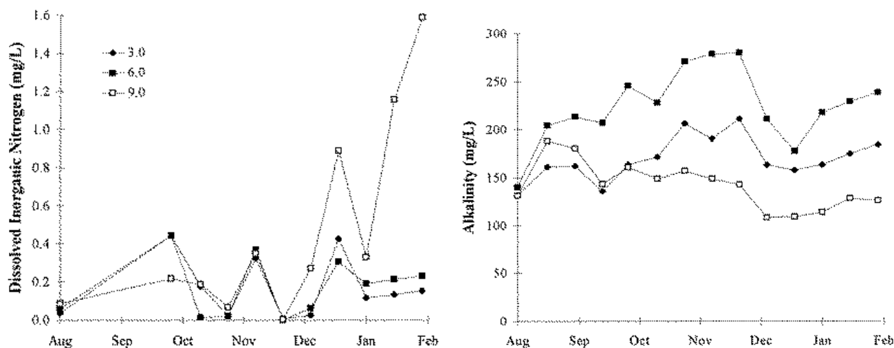
Figure 4. Changes in dissolved inorganic nitrogen and alkalinity during culture in each treatment.
