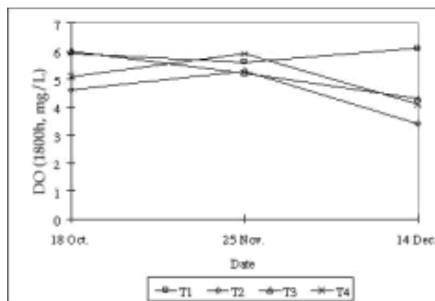
Figure 8. Mean dissolved oxygen (DO) concentration (mg/l) at 1800 h measured at different dates in different treatments.
