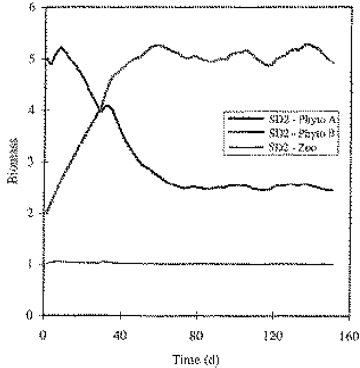
Figure 7. Biomass of the two pools of phytoplankton (in \text{g C m}^{-3} ) and that of zooplankton ( \text{g m}^{-1} ) predicted by Level 2 models in Nile tilapia ponds stocked at 2 \text{ fish m}^{-2} .
