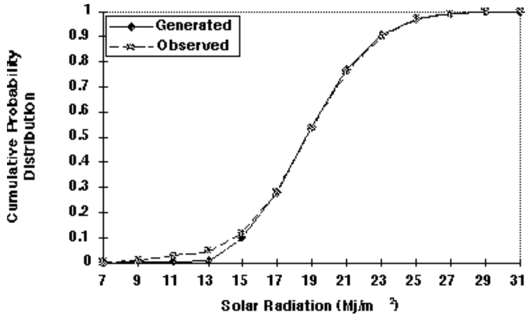
Figure 1. Comparison of the cumulative probability distribution curves between the generated and measured data.
