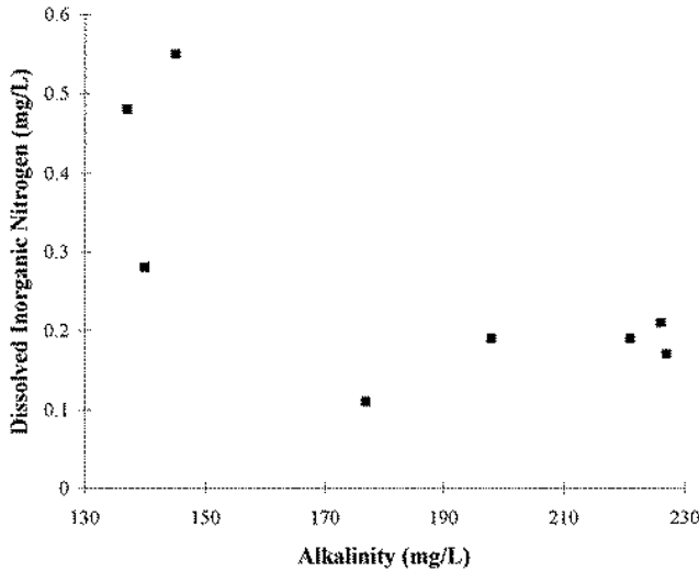
Figure 5. Relationship between alkalinity and dissolved inorganic nitrogen in ponds of all treatments.
