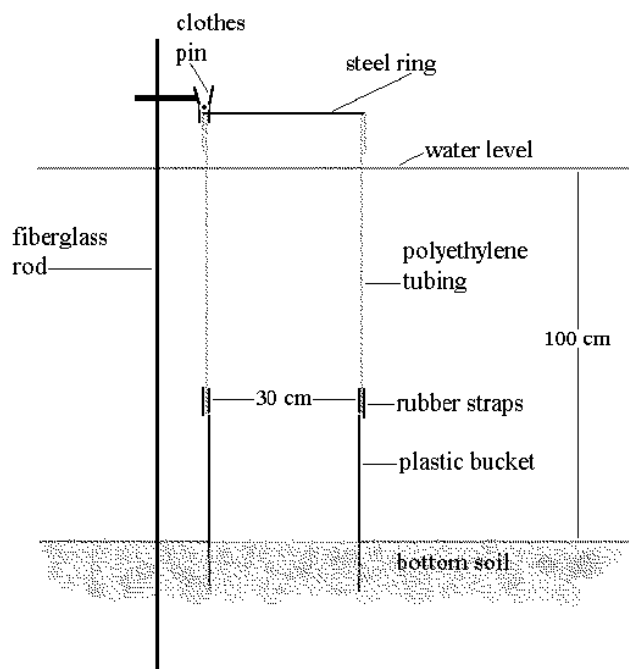
Figure 1. Design (not drawn to scale) of the artificial enclosures (isolation columns) used in the study. All materials used were locally available with the exception of the “layflat”, polyethylene tubing ordered from a plastics distributor.
