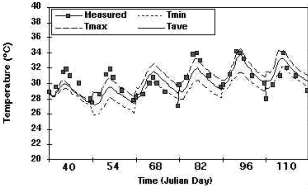
Figure 3. The generated maximum, minimum, and mean temperatures for the top pond layer are compared to the measured hourly data on Julian day 40, 54, 68, 82, 96, and 110.
