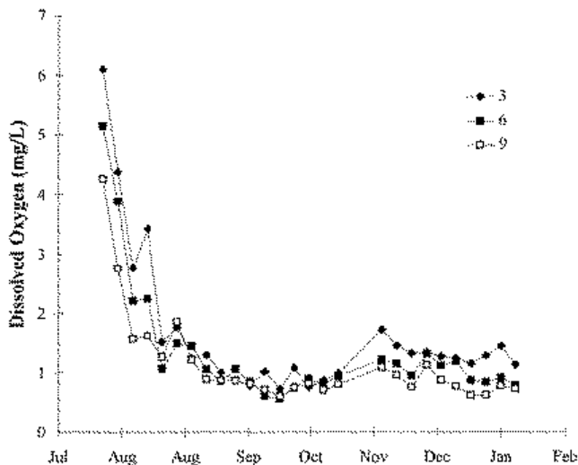
Figure 3. Changes in dissolved oxygen content of pond water during culture in each treatment.
