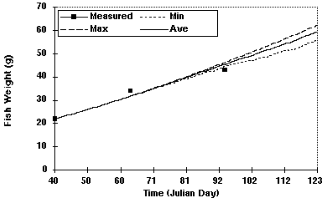
Figure 9. The generated maximum, minimum, and mean individual fish weight are compared to the measured data on Julian day 40, 64, and 97.
