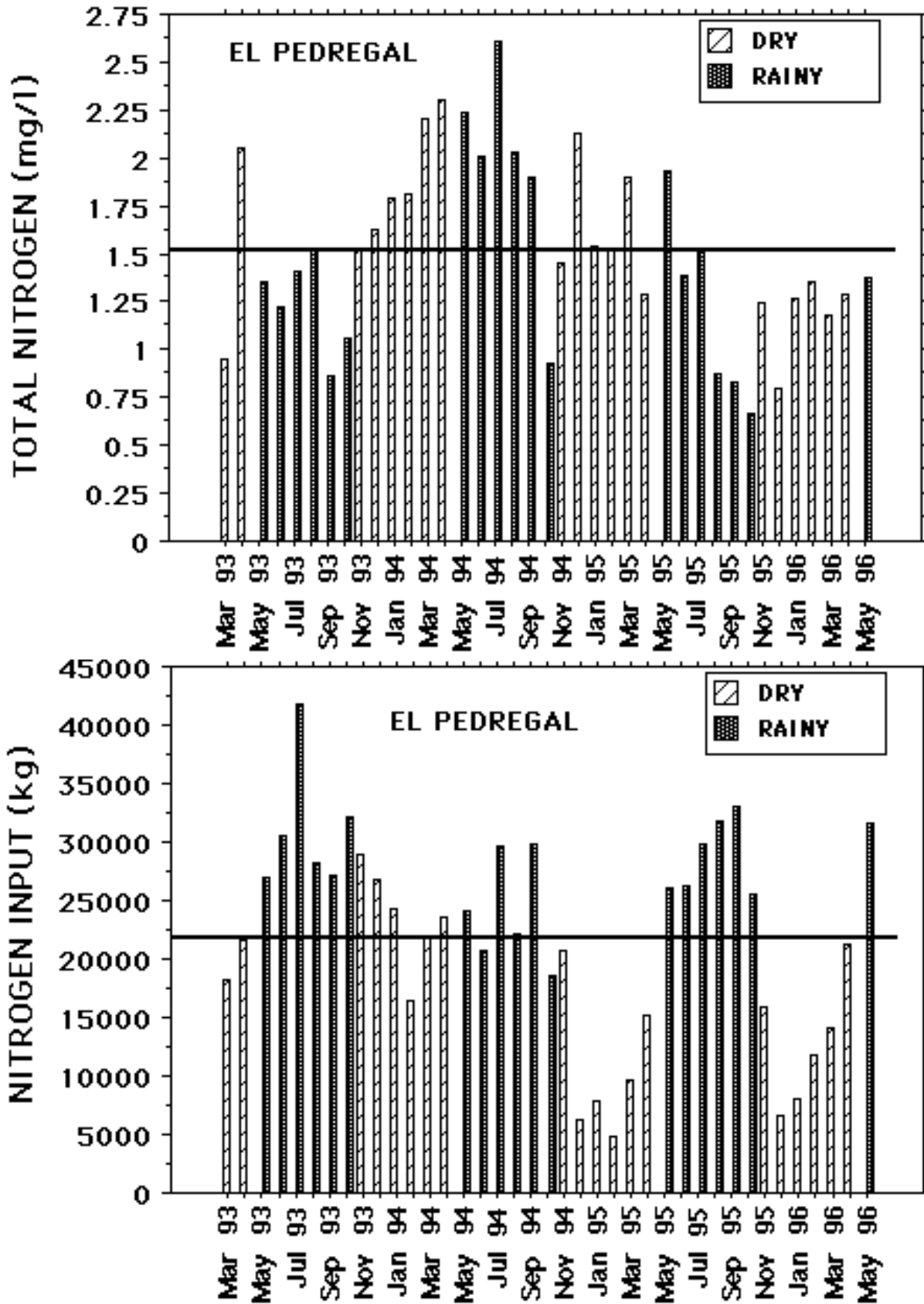
Figure 1. Mean monthly total nitrogen concentrations and nitrogen input as feed in El Pedregal estuary from March 1993 to May 1996. The horizontal black line is the mean during the sampling period.
