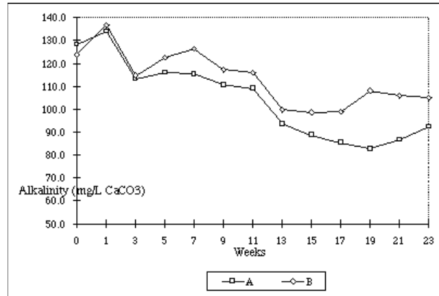
Figure 2. Fluctuation of alkalinity (mg/l \text{CaCO}_3 ) in both treatments over the culture period.
