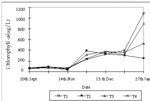
Figure 5. Mean chlorophyll-a concentration (µg/l) measured at different dates in different treatments.
