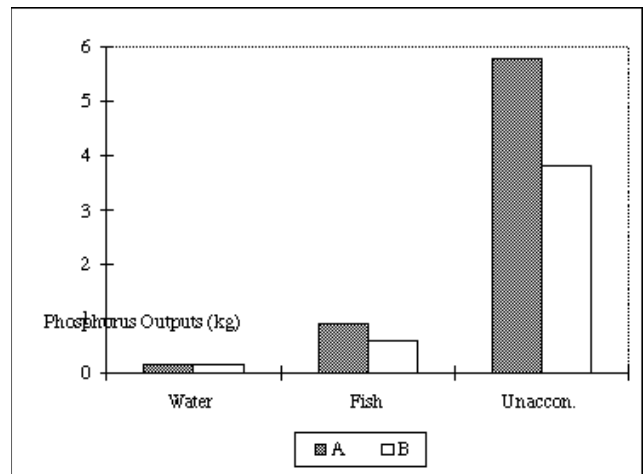
Figure 10. Comparison of phosphorus losses (kg) in both treatments over the culture period.
