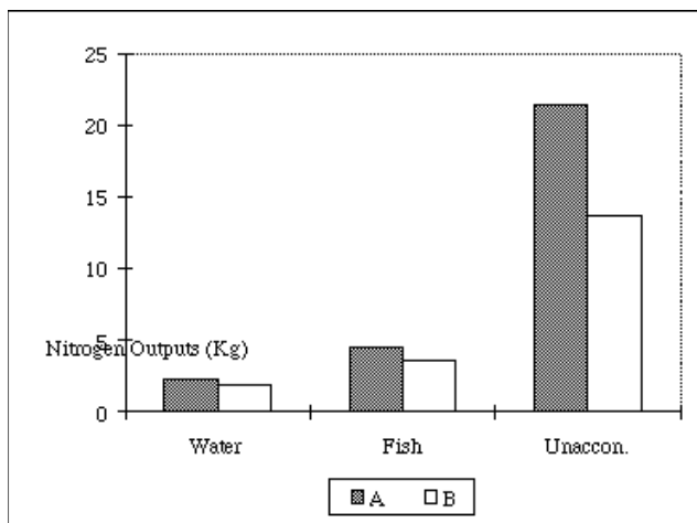
Figure 9. Comparison of nitrogen losses (kg) in both treatments over the culture period.
