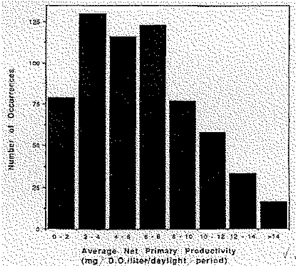
Figure 1. Frequency of average NPP extracted from the CRSP Central DataBase. Each occurrence is the average NPP for a pond during an experiment.
