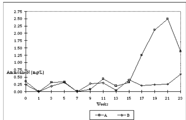
Figure 3. Fluctuation of total ammonia nitrogen (mg/l) in both treatments over the culture period.
