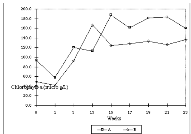
Figure 4. Fluctuation of Chlorophyll- a ( \mu\text{g/l} ) in both treatments over the culture period.
