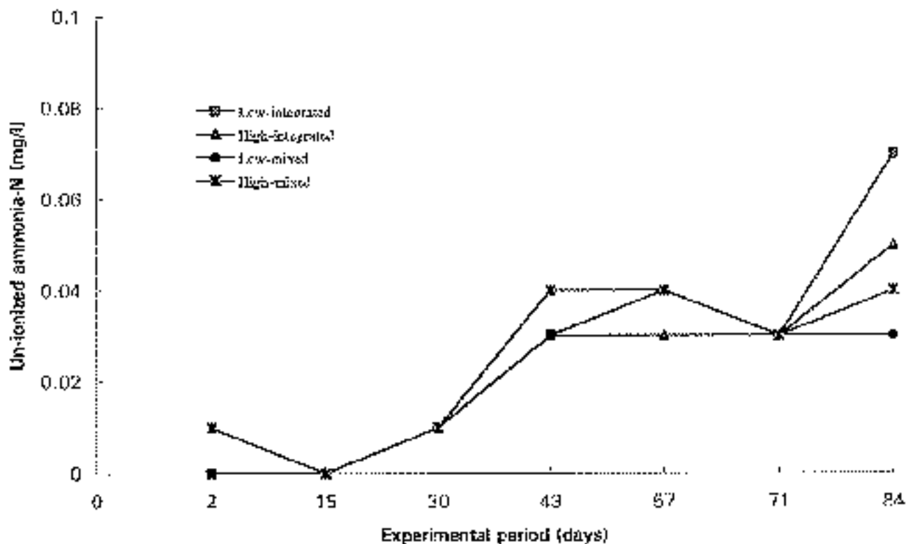
Figure 4. Fluctuations in un-ionized ammonia nitrogen at 0900 hr in all treatments throughout the experimental period.
