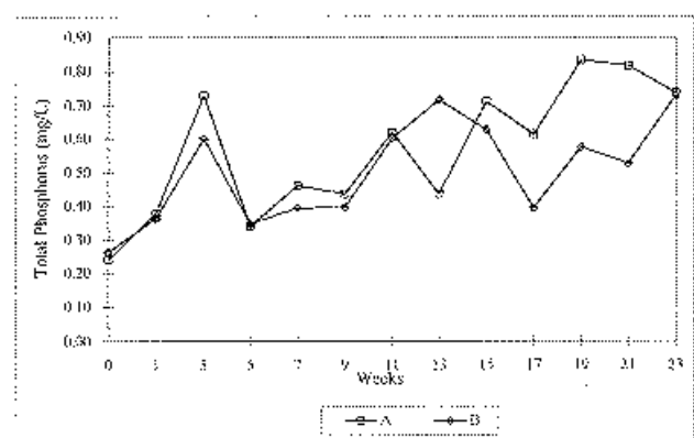
Figure 6. Fluctuation of total phosphorus (mg/l) in both treatments over the culture period.
