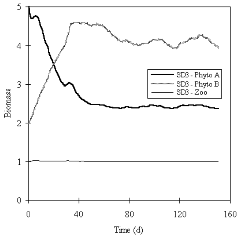
Figure 8. Biomass of the two pools of phytoplankton (in \text{g C m}^{-3} ) and that of zooplankton ( \text{g m}^{-1} ) predicted by Level 2 models in Nile tilapia ponds stocked at 3 \text{ fish m}^{-2} .
