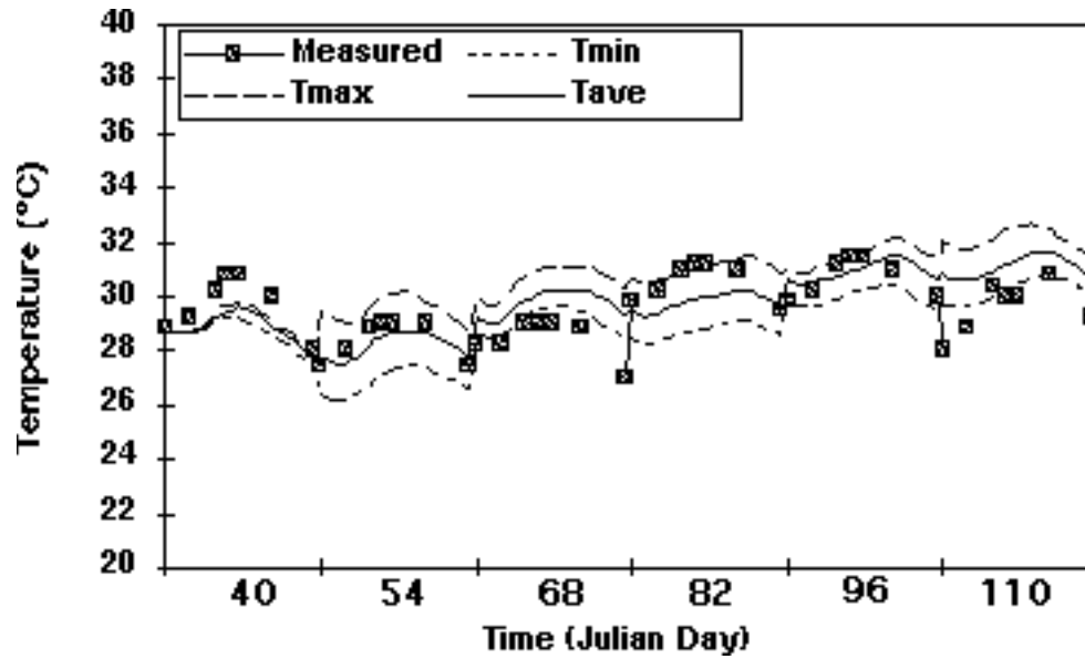
Figure 5. The generated maximum, minimum, and mean temperatures for the bottom layer are compared to the measured hourly data on Julian day 40, 54, 68, 82, 96, and 110.
