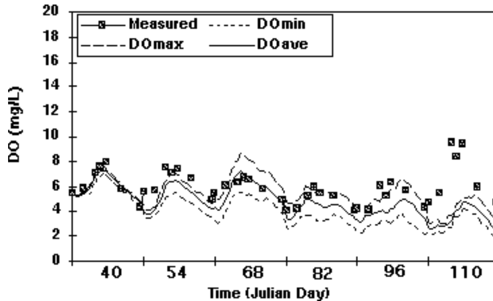
Figure 8. The generated maximum, minimum, and mean DO for the bottom layer are compared to the measured hourly data on Julian day 40, 54, 68, 82, 96, and 110.
