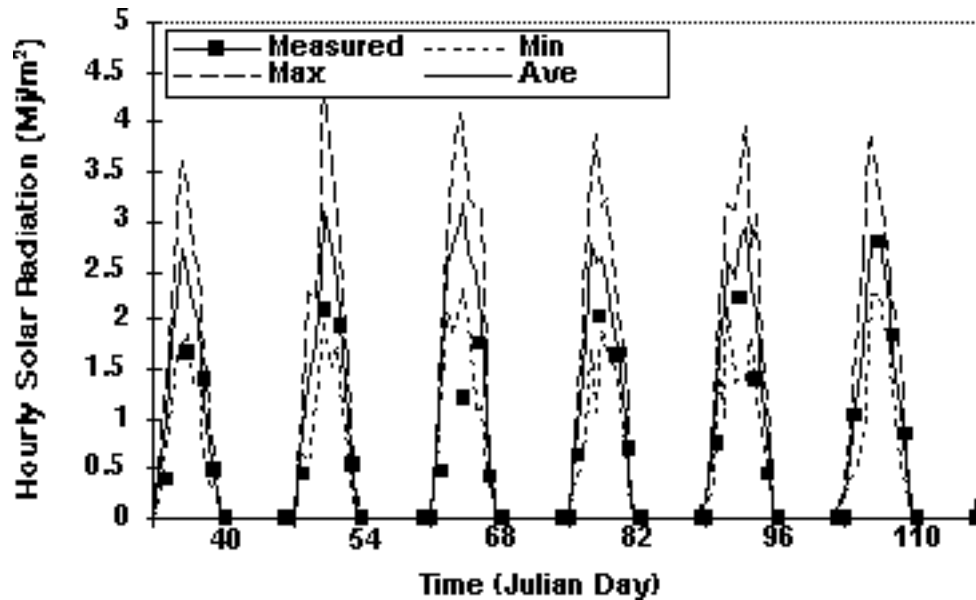
Figure 2. The generated hourly solar radiation values are compared to the measured hourly values on Julian day 40, 54, 68, 82, 96, and 110.
