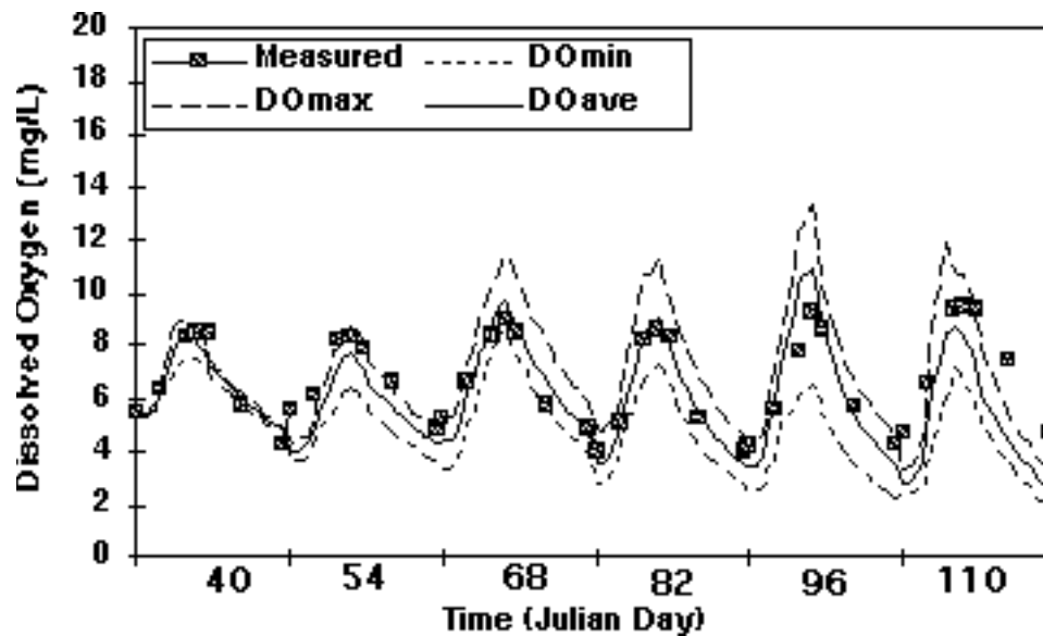
Figure 6. The generated maximum, minimum, and mean DO for the top layer are compared to the measured hourly data on Julian day 40, 54, 68, 82, 96, and 110.
