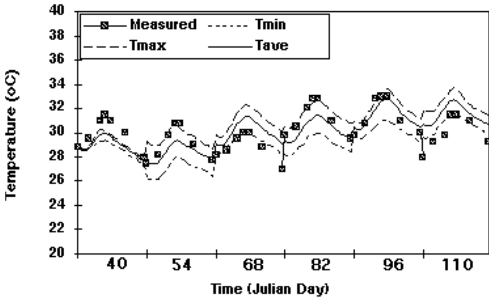
Figure 4. The generated maximum, minimum, and mean temperatures for the middle layer are compared to the measured hourly data on Julian day 40, 54, 68, 82, 96, and 110.
