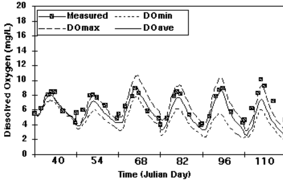
Figure 7. The generated maximum, minimum, and mean DO for the middle layer are compared to the measured hourly data on Julian day 40, 54, 68, 82, 96, and 110.
