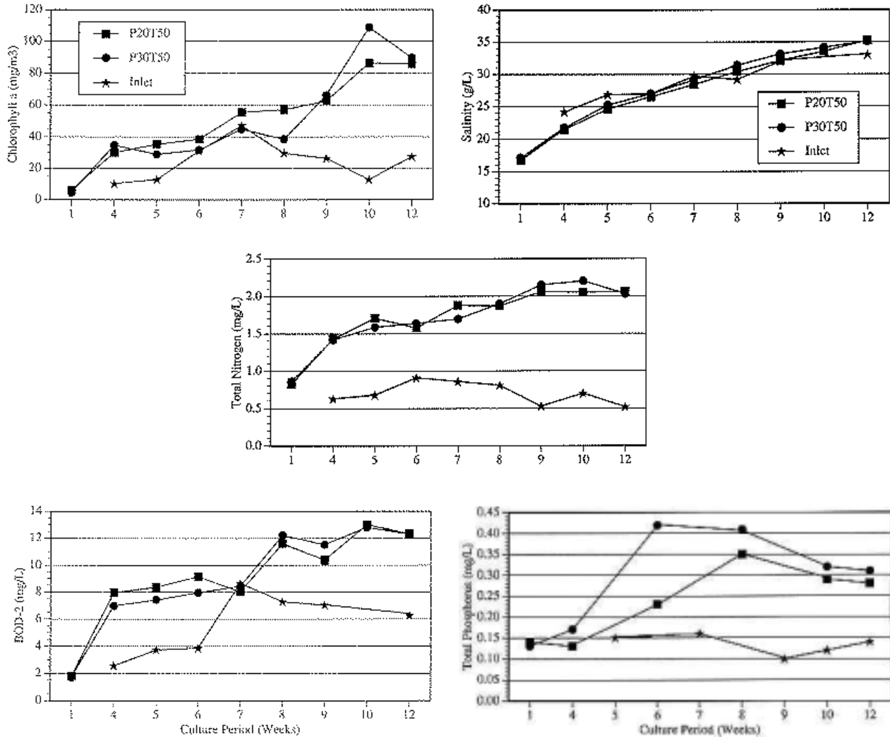
Figure 1. Mean weekly concentrations of 5 variables in ponds receiving a 20% protein (P20T50) or a 30% protein (P30T50) feed, and in inlet water.
