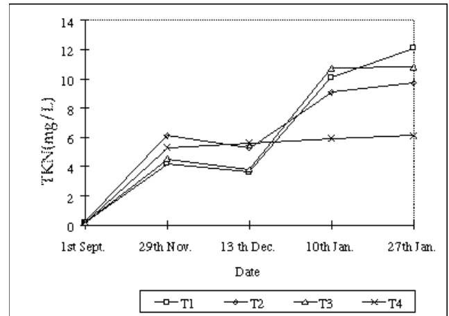
Figure 2. Mean total kjeldahl nitrogen (TKN) (mg/l) measured at different dates in different treatments.
