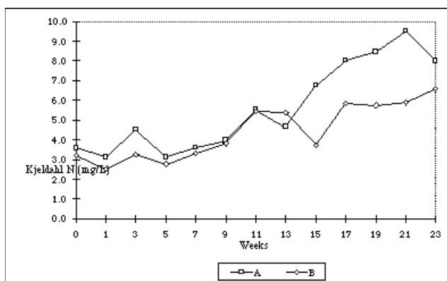
Figure 5. Fluctuation of total Kjeldahl nitrogen in both treatments over the culture period.
