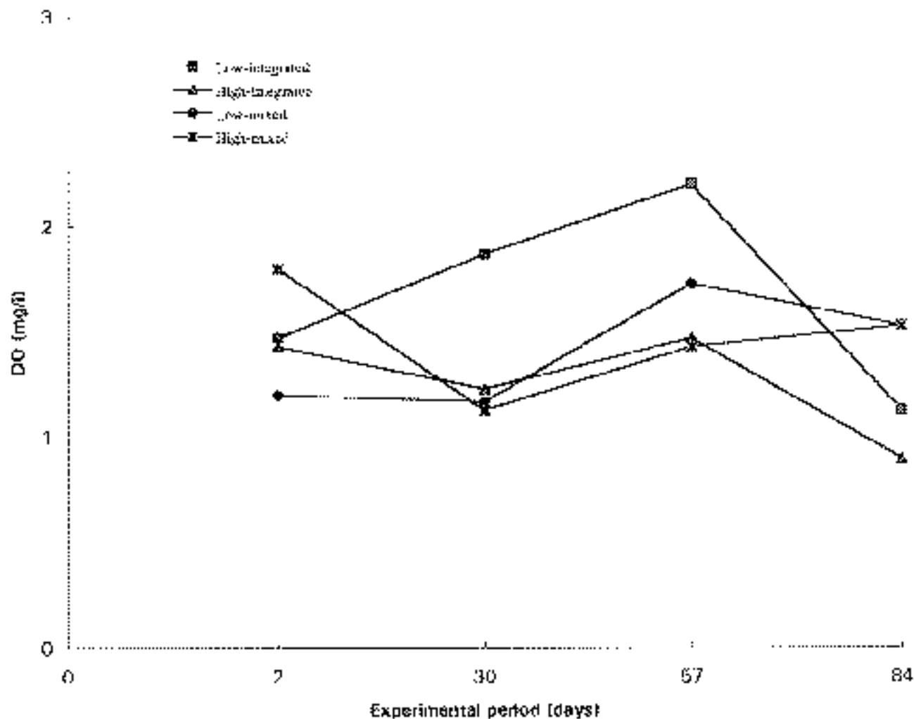
Figure 3. Fluctuations in DO at dawn in all treatments throughout the experimental period.
