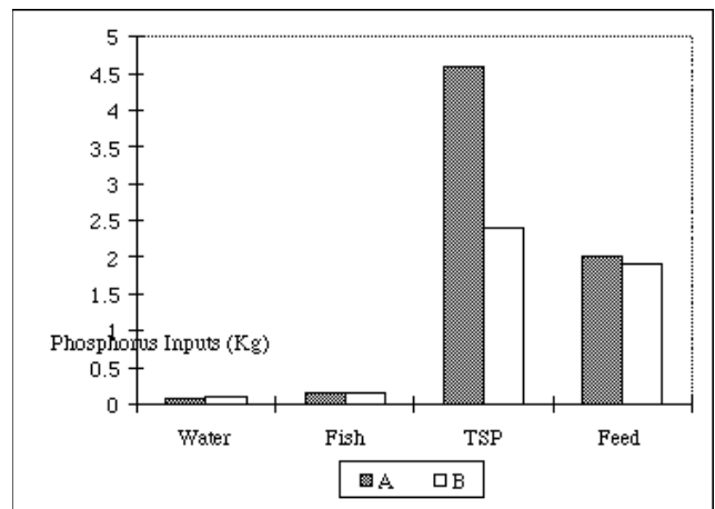
Figure 8. Comparison of phosphorus inputs (kg) in both treatments over the culture period.
