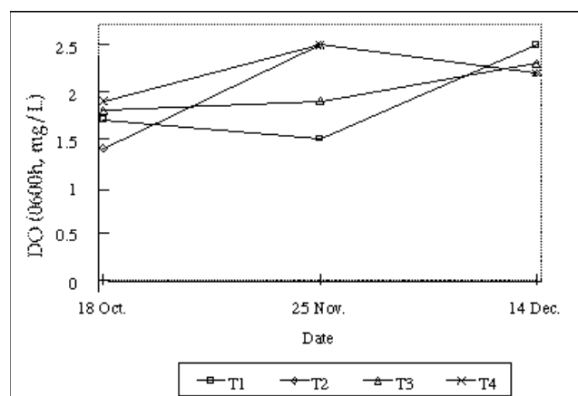
Figure 7. Mean dissolved oxygen (DO) concentration (mg/l) at 0600 h measured at different dates in different treatments.
