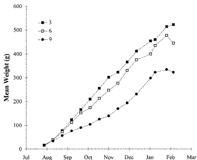
Figure 1. Changes in mean weight of tilapia during culture under three treatments.
