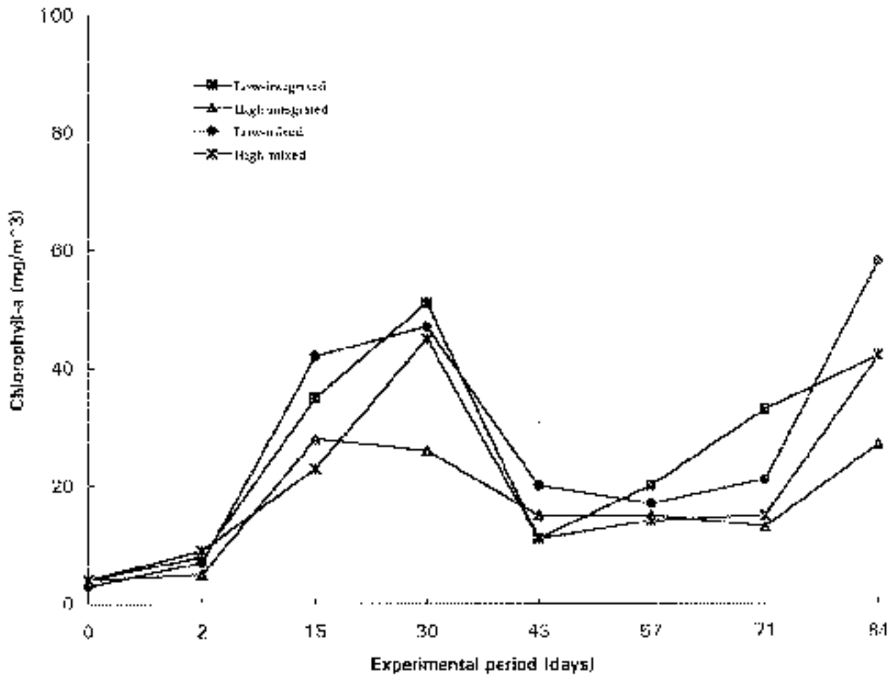
Figure 5. Fluctuations in chlorophyll-a at 0900 hr in all treatments throughout the experimental period.
