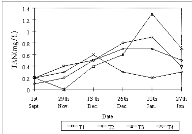
Figure 1. Mean total ammonia nitrogen (TAN) (mg/l) measured at different dates in different treatments.
