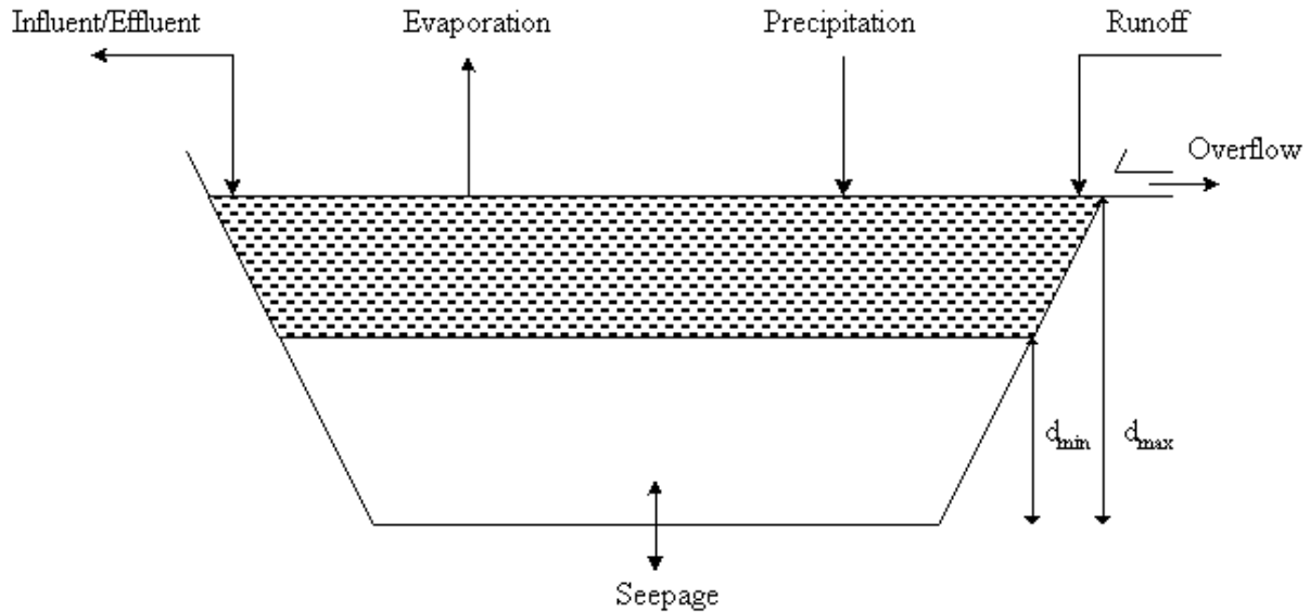
Figure 1. Schematic diagram showing the types of water sources and sinks that can be considered in the POND® water budget model, d_{\min} and d_{\max} respectively refer to the minimum desired and maximum possible pond water depth.
