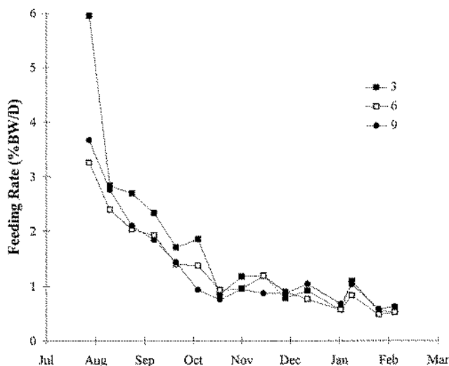
Figure 2. Changes in feeding rate and feed conversion rate during culture for ponds in each treatment.
