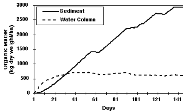
Figure 4. Water column and sediment organic matter predicted using the multi-G organic matter model.
