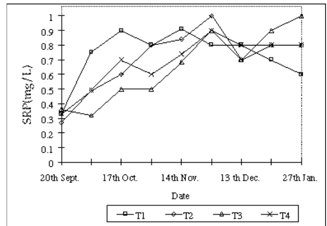
Figure 4. Mean soluble reactive phosphorus (SRP) (mg/l) measured at different dates in different treatments.
