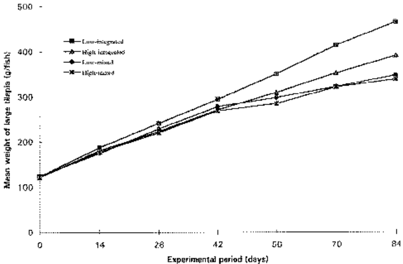
Figure 1. Growth of large Nile tilapia in the integrated and mixed pond culture systems over the experimental period.
