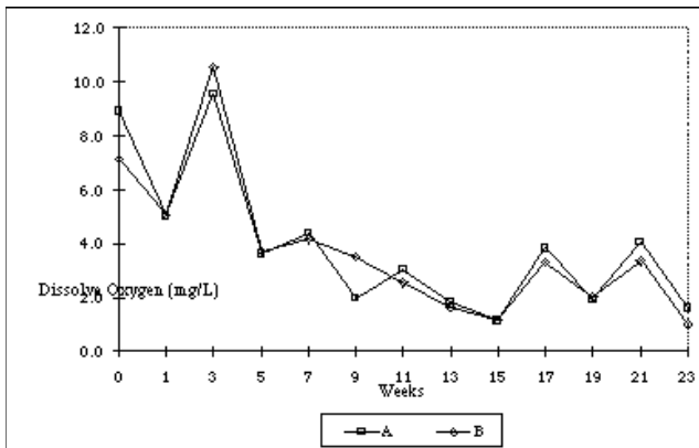
Figure 1. Fluctuation of dissolved oxygen (mg/l) in both treatments over the culture period.
