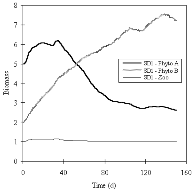
Figure 6. Biomass of the two pools of phytoplankton (in g C m -3 ) and that of zooplankton (g m -1 ) predicted by Level 2 models in Nile tilapia ponds stocked at 1 fish m -2 .
