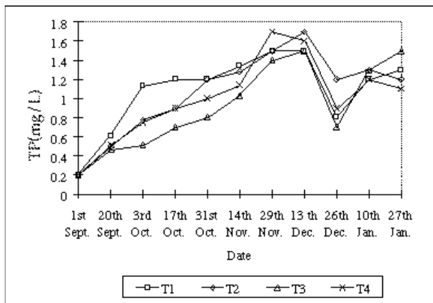
Figure 3. Mean total phosphorus (TP) (mg/l) measured at different dates in different treatments.
