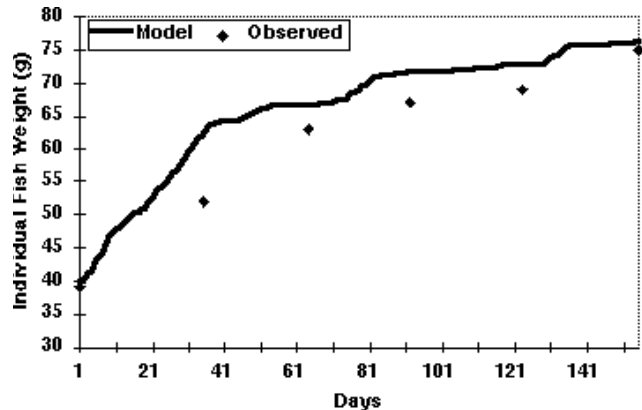
Figure 3. Fish weight predicted by the modified bioenergetics model for the Butare site in Rwanda.
